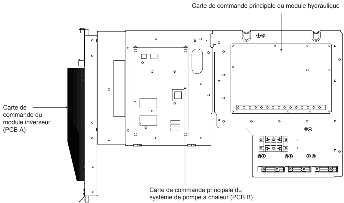
12/14/16kW (1-phase)
