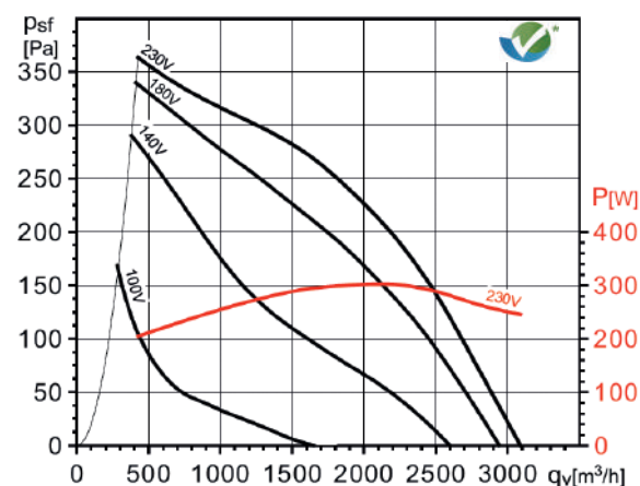
CRHB/4-355
