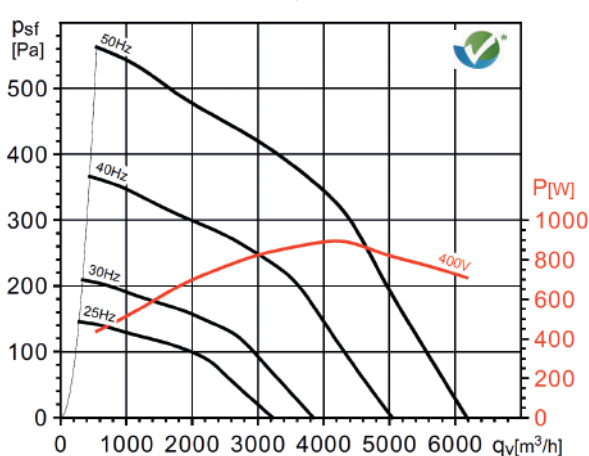
CRHT/4-450
