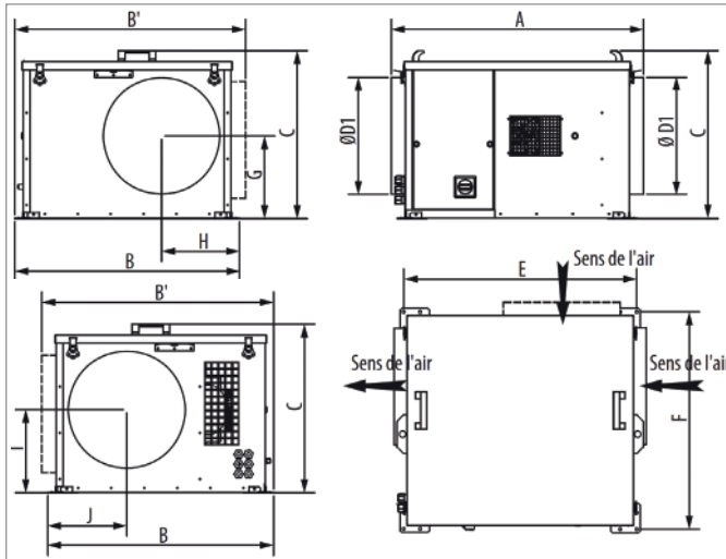
CRCB ECOWATT L/M - REFOULEMENT HORIZONTAL
