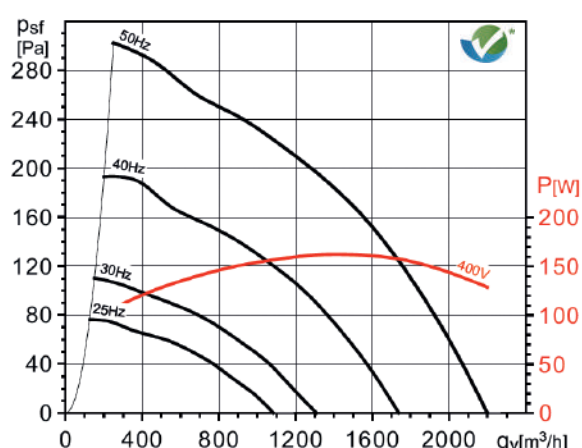
CRHT/6-315
