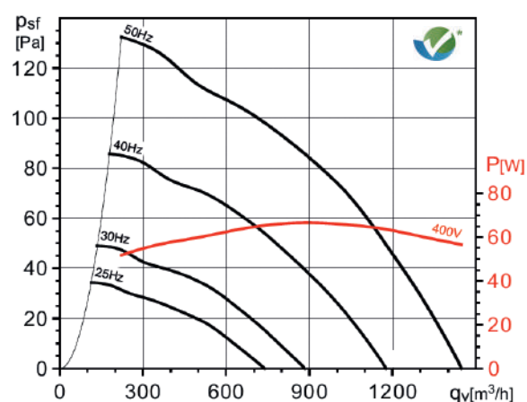
CRHT/4-355
