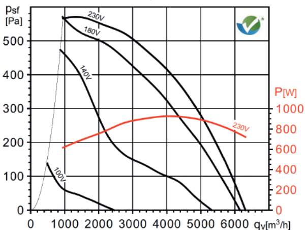
CRHB/4-450
