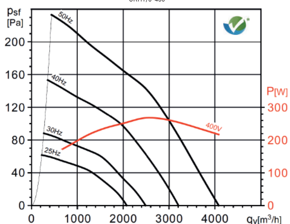
CRHT/6-450
