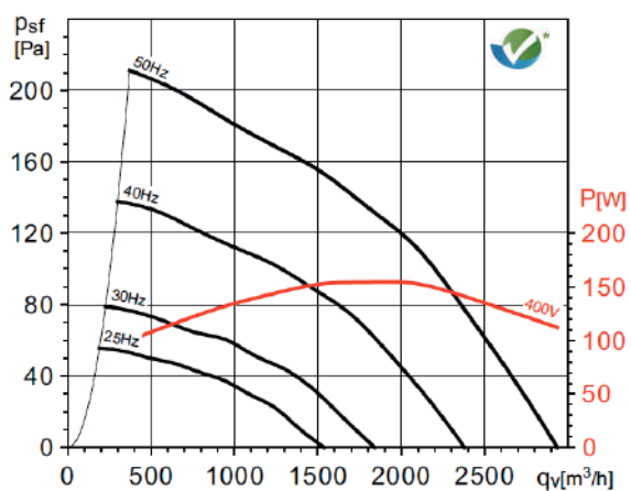
CRHT/6-400
