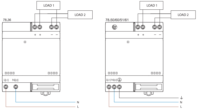
Raccordement double
