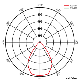
Empotrar S069L0P Embed S069L0P Empotrate S069L0P Empotrare S069L0P
